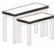
TB 100-R Nesting Tables with Riser 48" L x 30" W x 36" H 36" L x 30" W x 24" H Riser: 30" L x 15" W x 10" H
