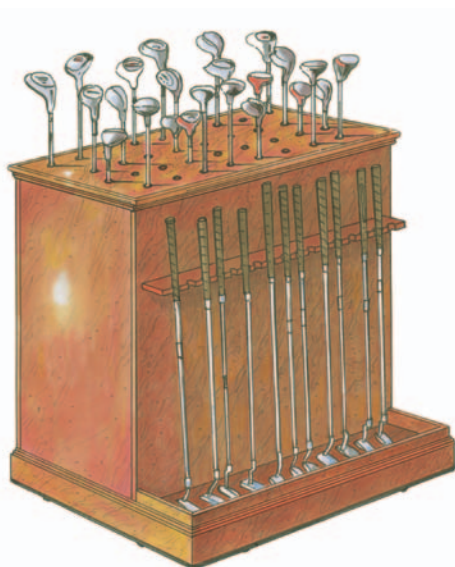
CL 102-47 Small Utility Club Display 42" H x 47" W x 34" D 34 Clubs in Top 17 Clubs in Grip Strip
